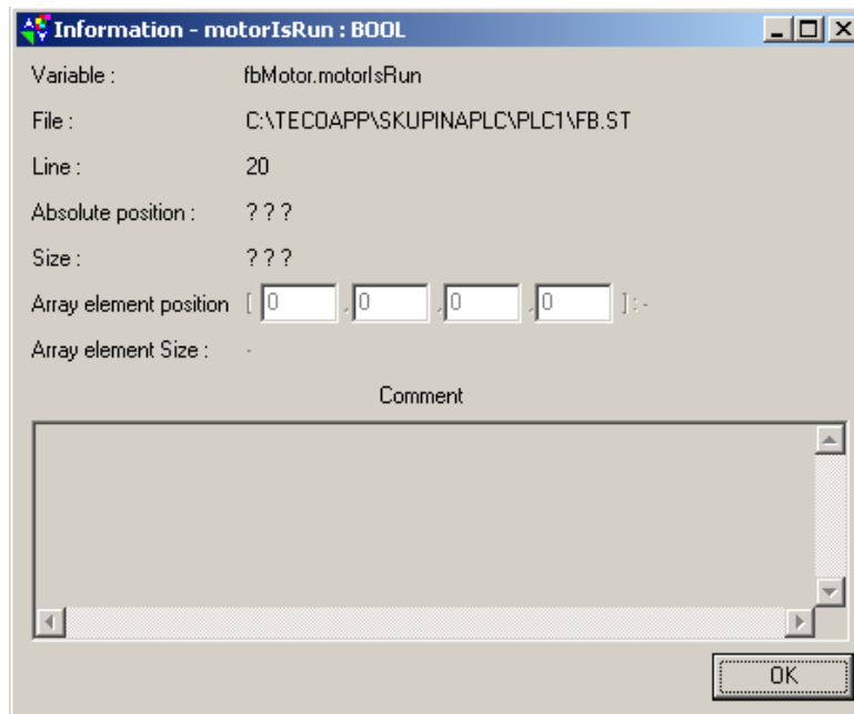
Fig. 36. Example of display of IEC manager item features
