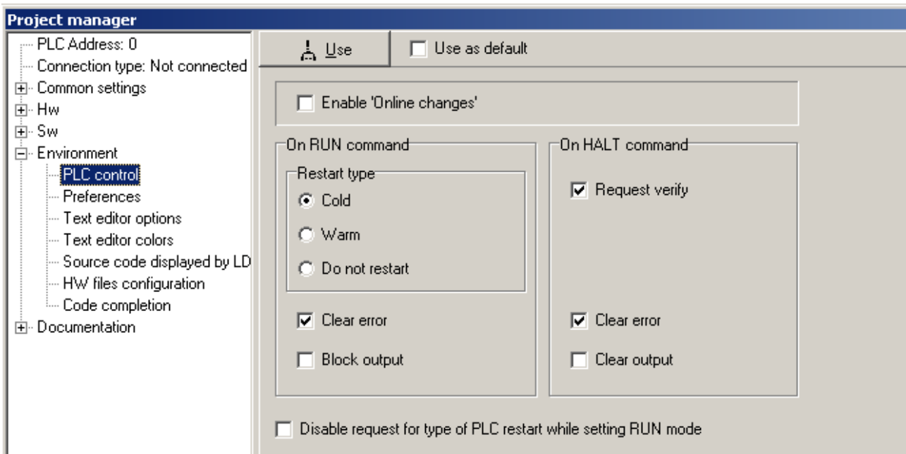
Fig. 31. PLC control window
