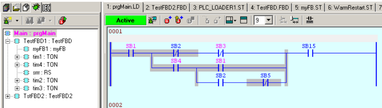
Fig. 83. Program debugging in LD language
