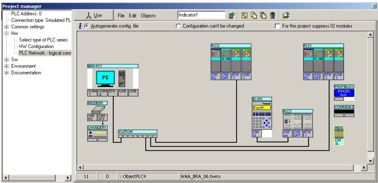
Fig. 25. Window for configuring the logic connection of a PLC and its environment
