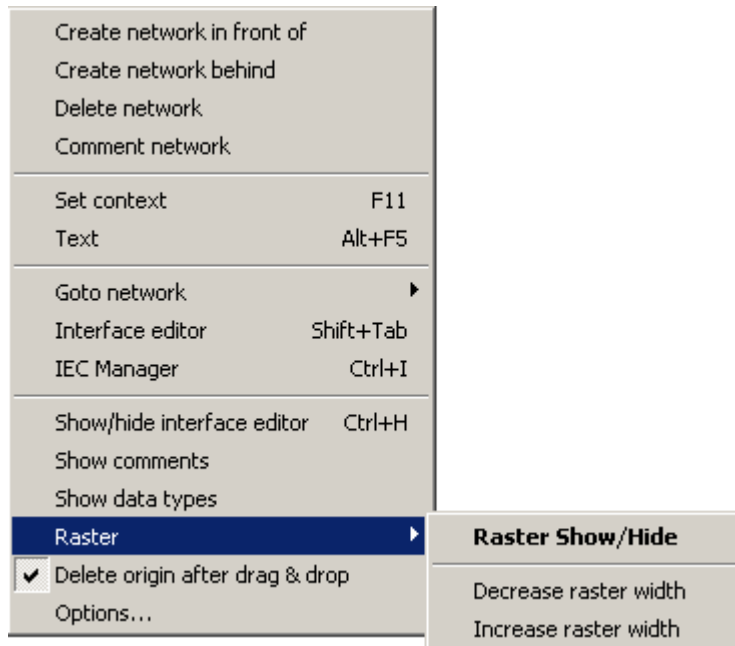
Fig. 63. Local menu in LD editor area
