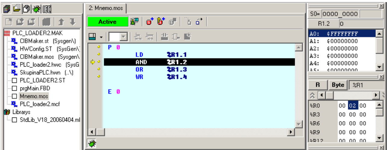
Fig. 85. Program debugging in mnemocode language
