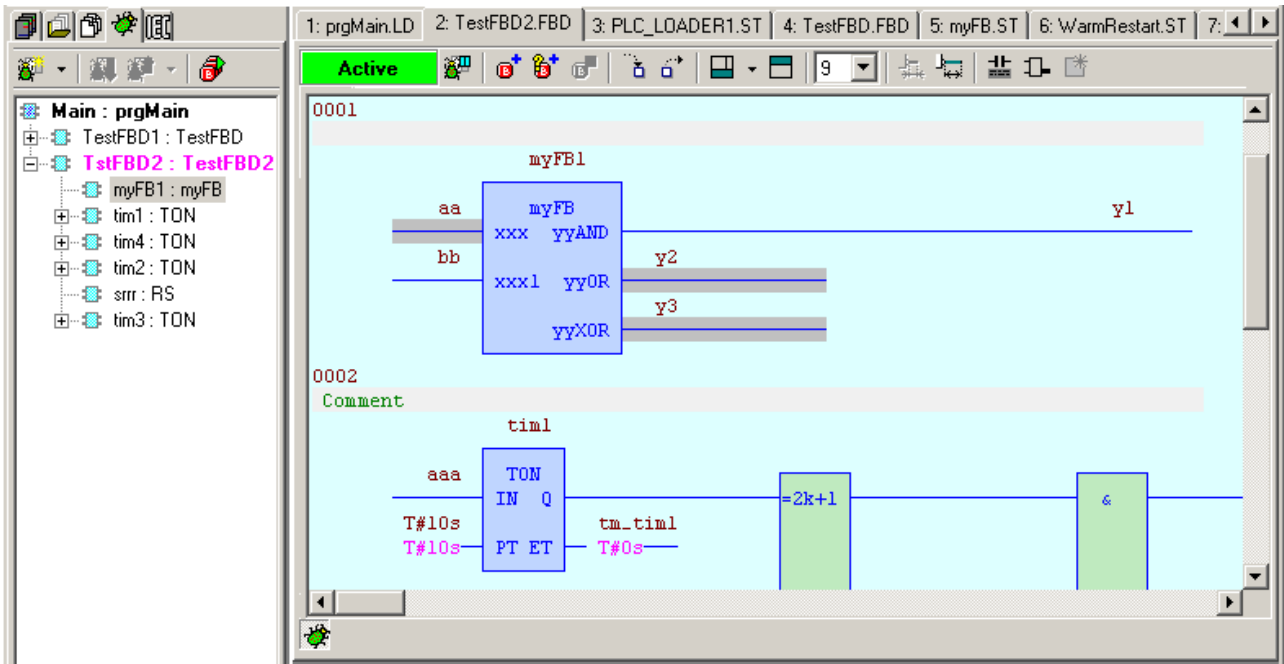
Fig. 84. Program debugging in FBD language
