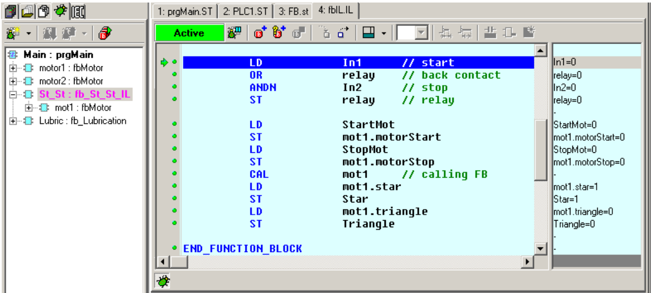
Fig. 82. Program debugging in IL language
