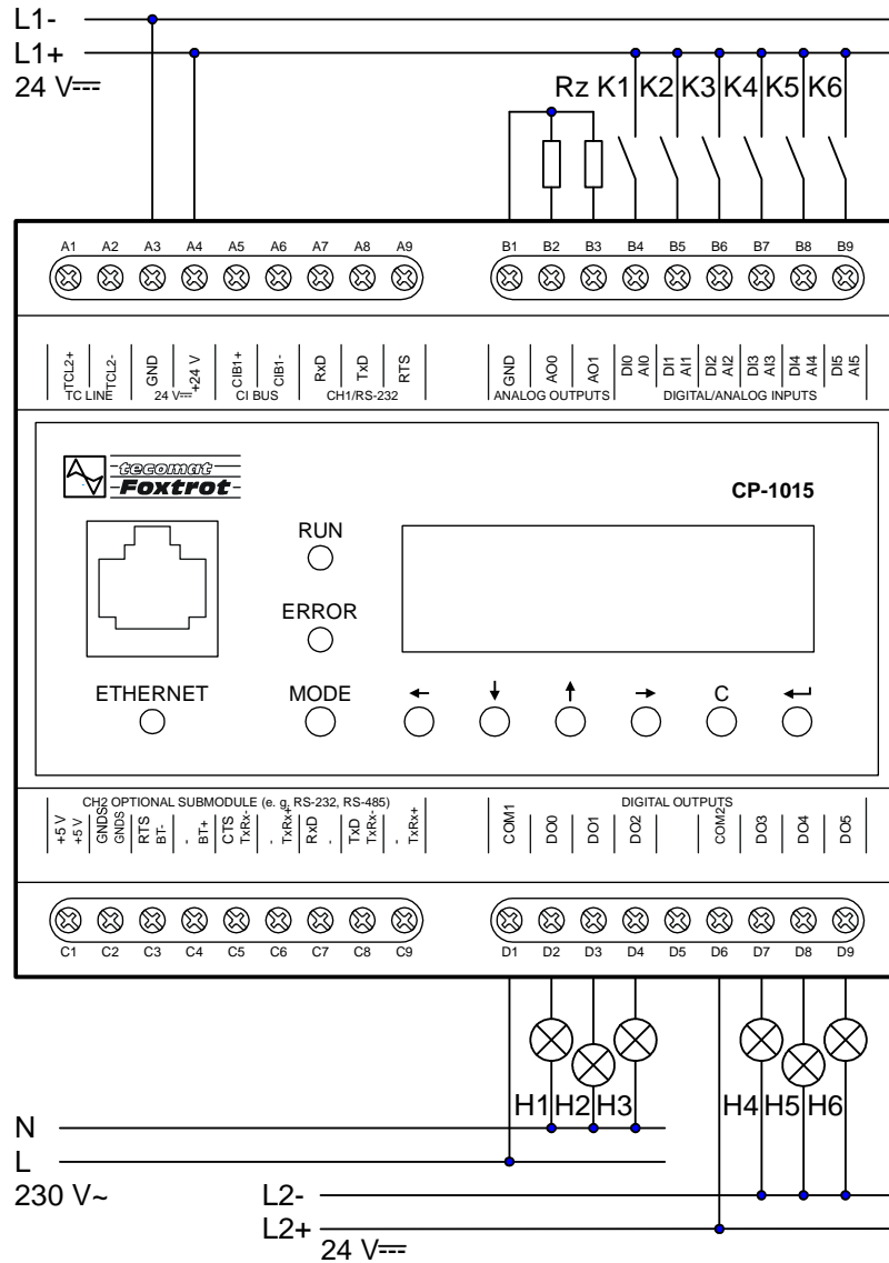
Fig. 4.1 Elementary connection of CP-1015 module
