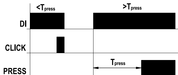
Fig. 3. 17 Evaluation of short / long press
