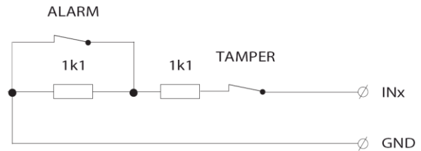
Fig. 3. 26 Double-balanced input for security detectors
