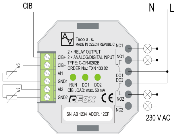
Fig. 3. 62 view C-OR-0202B
