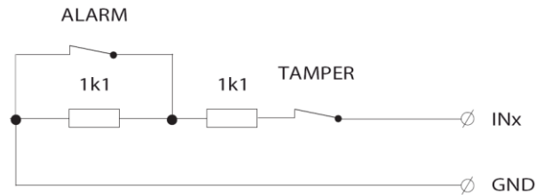
Fig. 3. 15 Double-balanced input for security detectors
