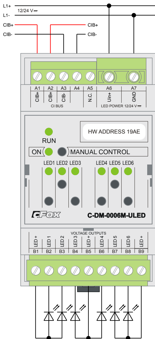
Fig. 3.22 View and connection C-DM-0006M-ULED
