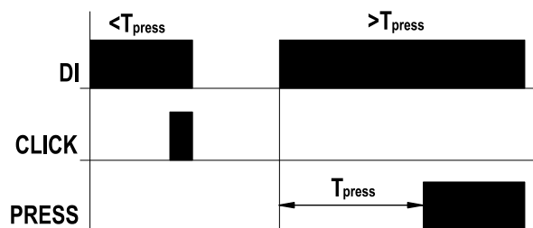
Fig. 3. 28 Evaluation of short / long press
