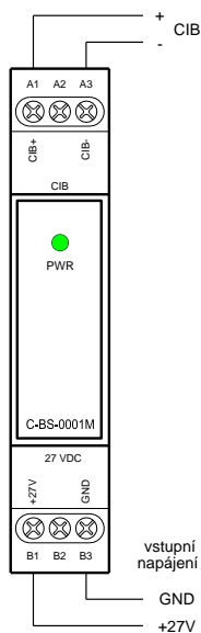
Fig. 2.12 Connection example C-BS-0001M
