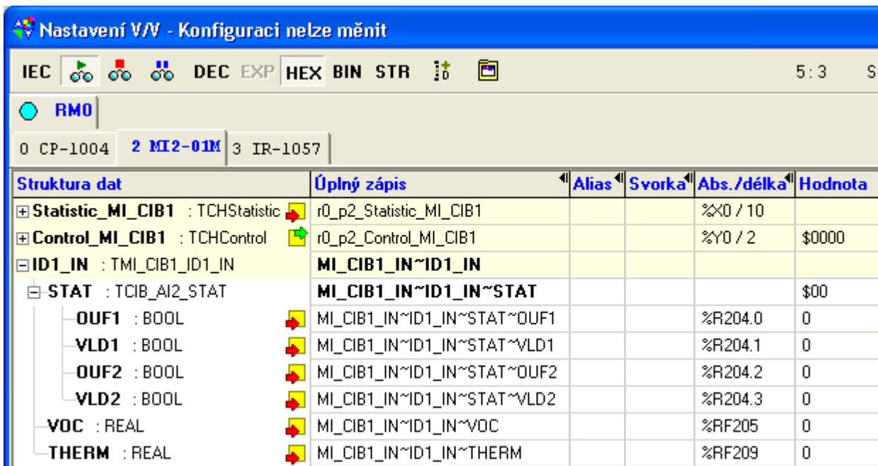
Fig. 3.9 The structure of the transmitted data
