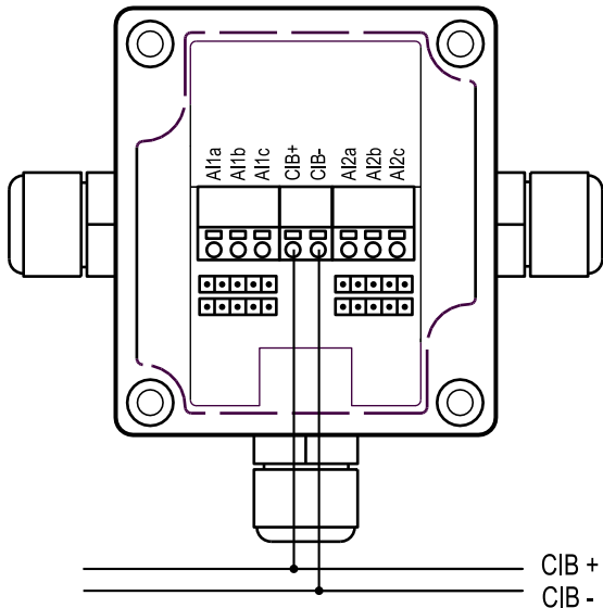
Fig. 3.36 View C-IT-0200I
